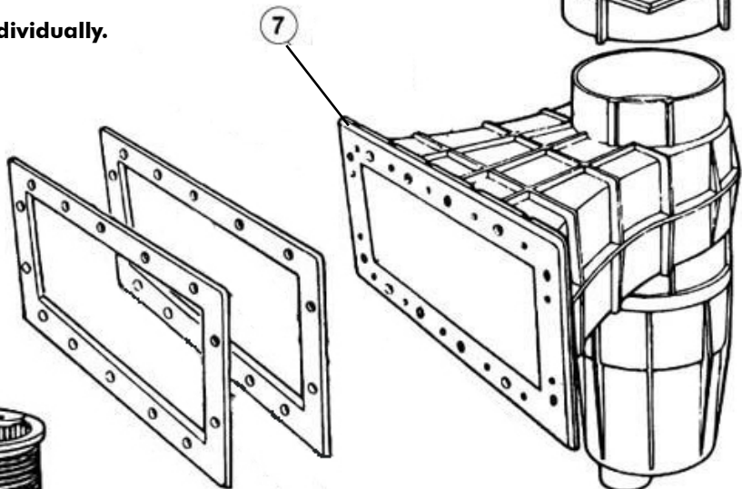
JACUZZI WWF SKIMMER PARTS BREAKDOWN
