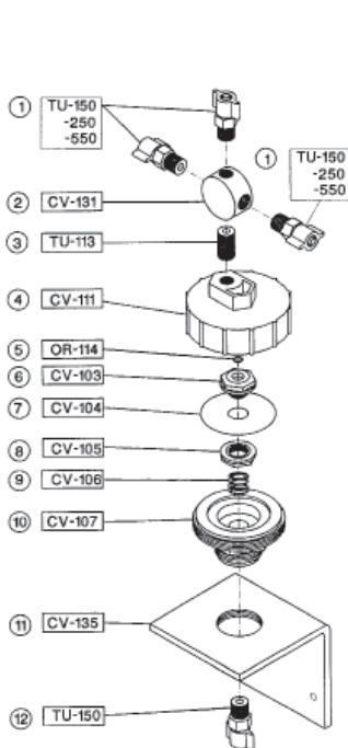
PRESSURE RELIEF/ VENT VALVE
