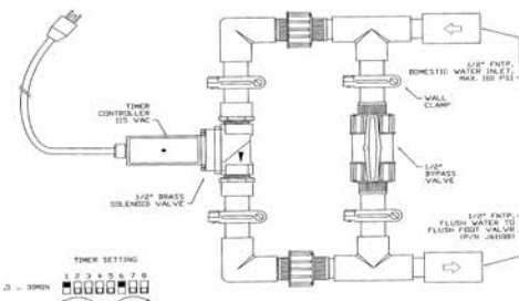
PULSATRON AUTO-FLUSH CONTROLLER
