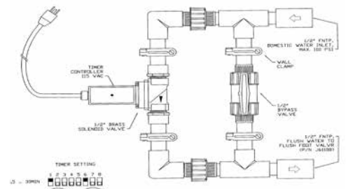
PULSATRON AUTO-FLUSH CONTROLLER
