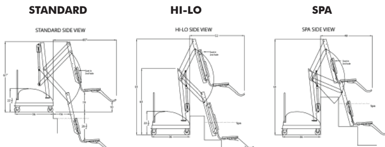
PAL PORTABLE AQUATIC LIFT DIMENSIONS
