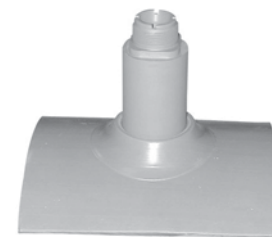
GLUE ON SADDLE
