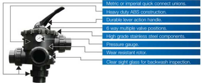
MICRON HORIZONTAL SAND FILTER
