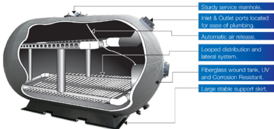
WATERCO HORIZONTAL SAND FILTER
